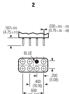
Terminals
